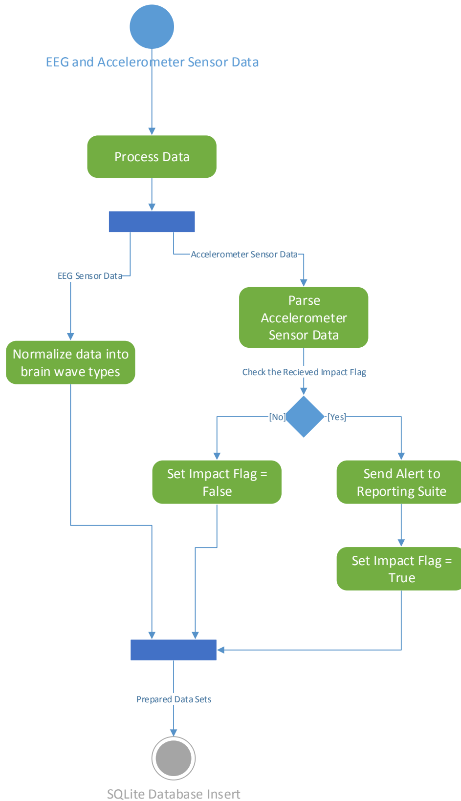
Figure 4-37: Data Preparation Activity Diagram; A UML activity diagram demonstrating the data preparation module of the data receiving Python script
