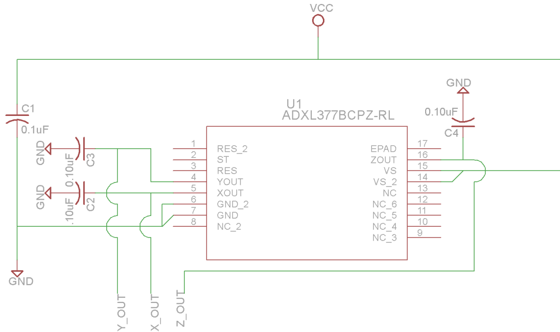
Figure 4-18: ADXL377 Schematic Design; An EagleCAD schematic design describing the ADXL377
