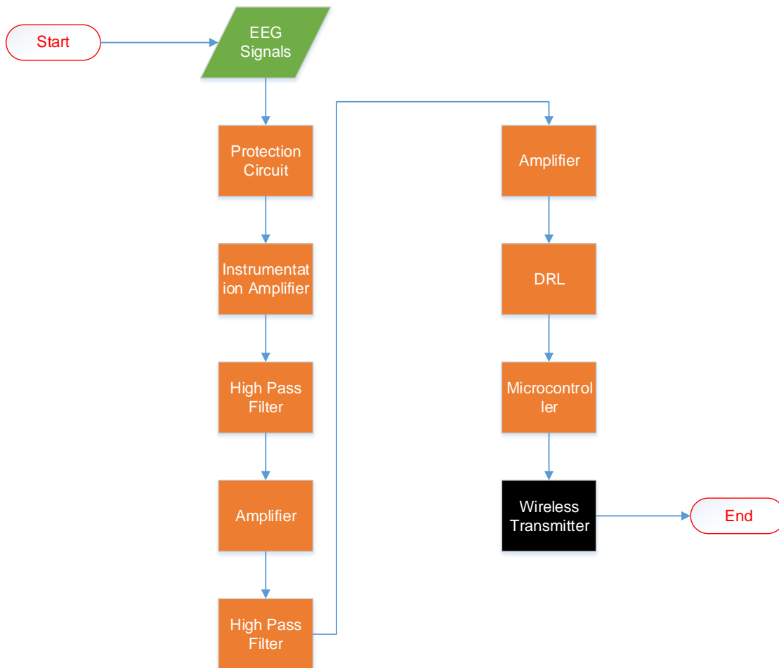
Figure 4-14: Final EEG Block Diagram; A block diagram representing the final EEG sensor array block diagram
