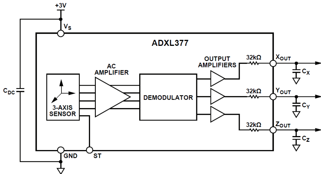
Figure 4-16: ADXL377 Block Diagram; A block diagram of the ADXL377 3-Axis High g Analog MEMS Accelerometer; reprinted with permission from Analog Devices, Inc.
