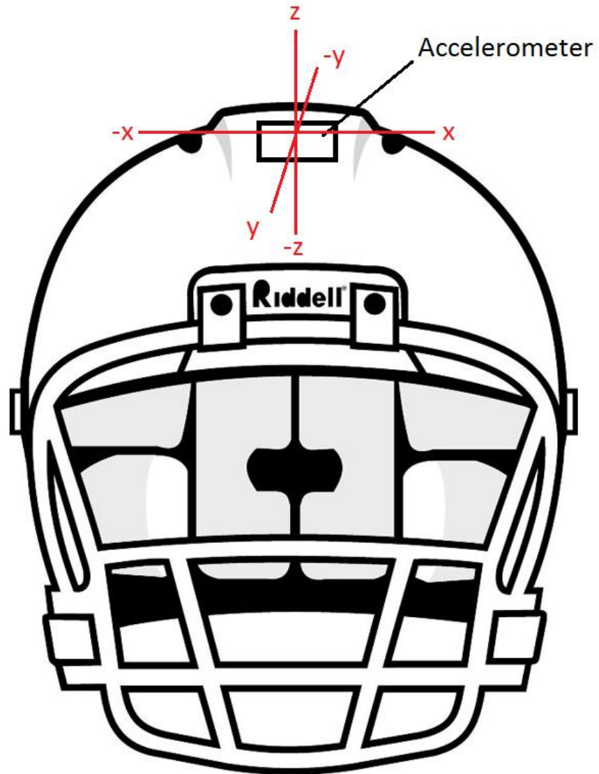
Figure 4-15: Accelerometer Helmet Mounting Location; A figure demonstrating the placement of the accelerometer sensor on the BIO-Helmet
