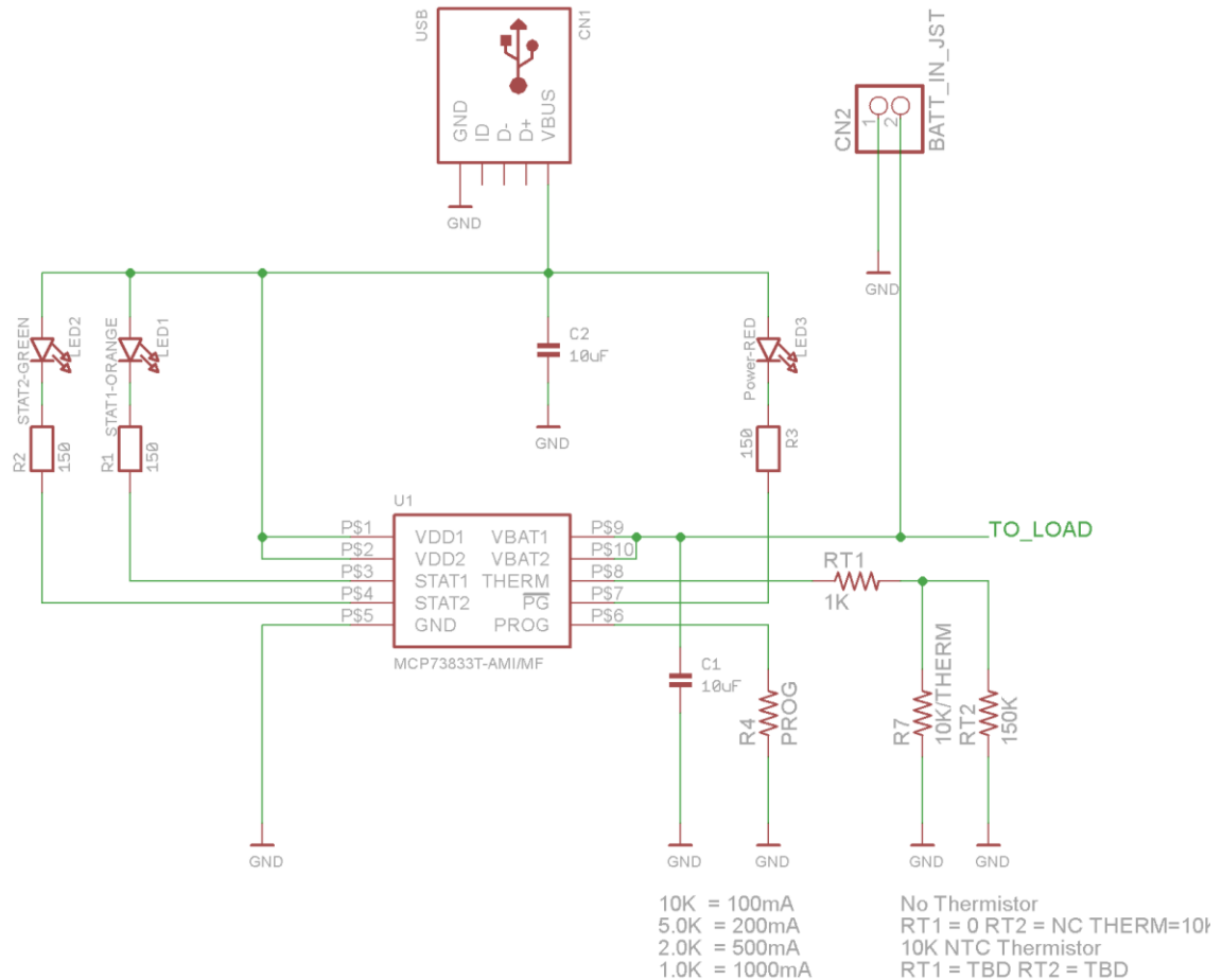
Figure 4-29: MCP73833/4 Charging Circuit; A schematic diagram detailing the battery charging using the MCP73833/4
