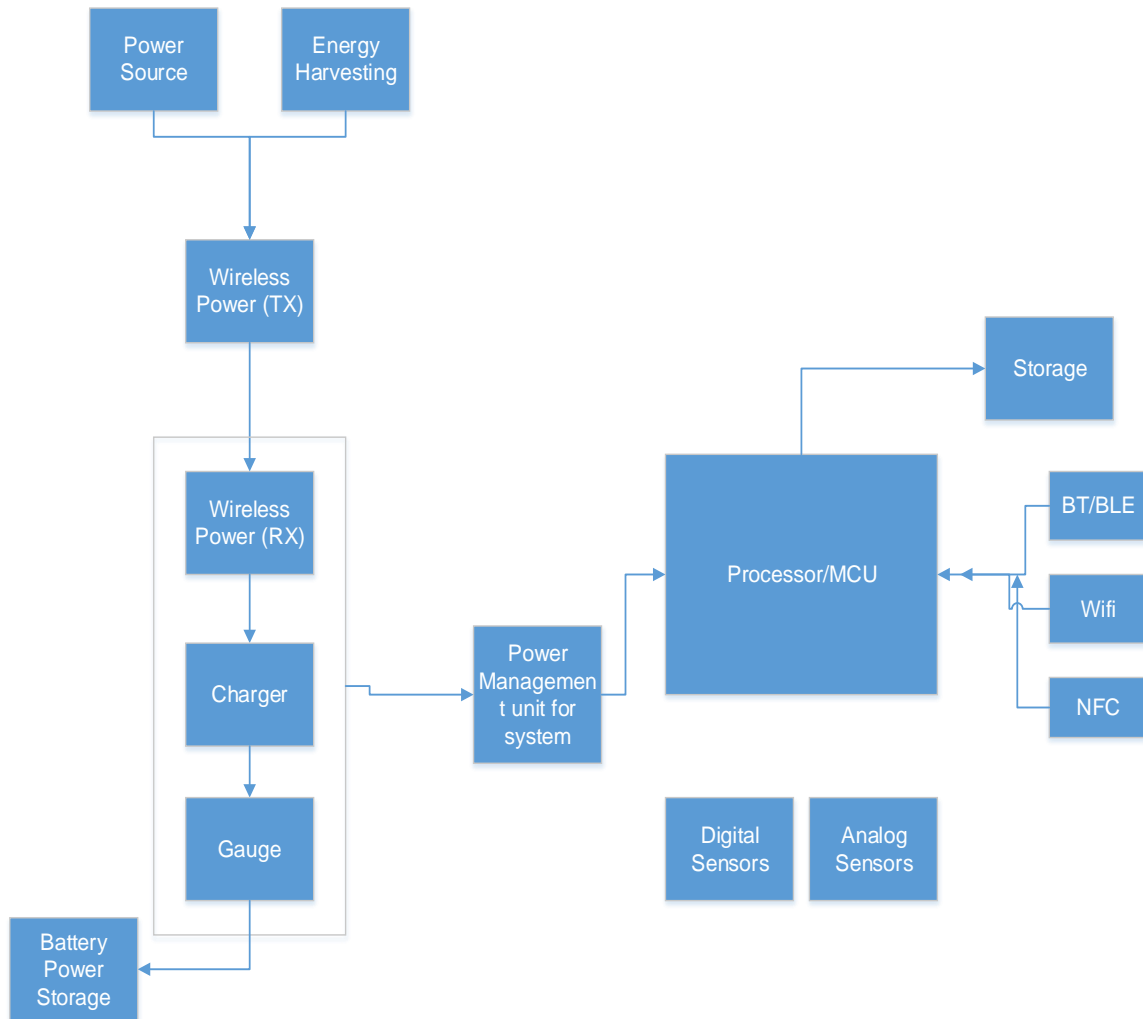
Figure 4-26: BIO-Helmet System Power Management; A figure describing the BIO-Helmet power management system
