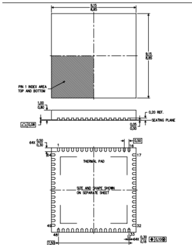
Figure 4-23: CC3100 Dimensions and Layout; A figure describing the size, dimensions, and layout of the CC3100; reprinted with permission from Texas Instruments, Inc.
