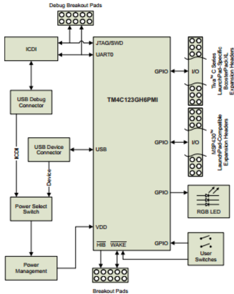
Figure 4-21: Tiva C TM4C123GH6PM; A figure demonstrating the overall layout of the TM4C123GH6PM microcontroller; reprinted with permission from Texas Instruments, Inc.
