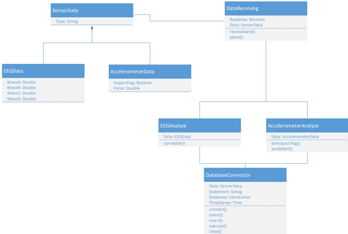
Figure 4-34: Data Receiving Class Diagram; A UML class diagram representing the BIO-Helmet data receiving Python script
