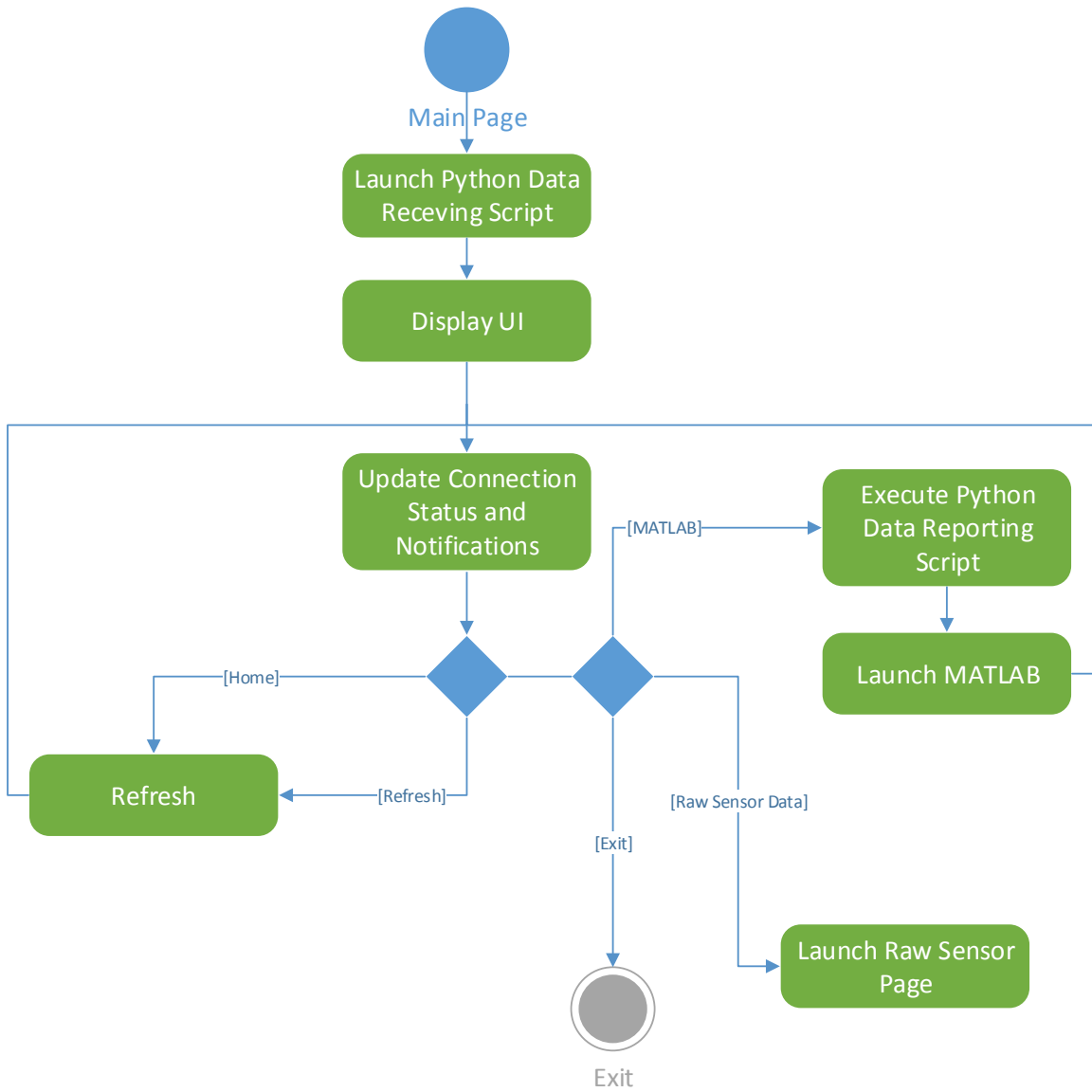
Figure 4-43: GUI Homepage; A UML activity diagram describing the user interface specific flow of the home page for the Python graphical user frontend
