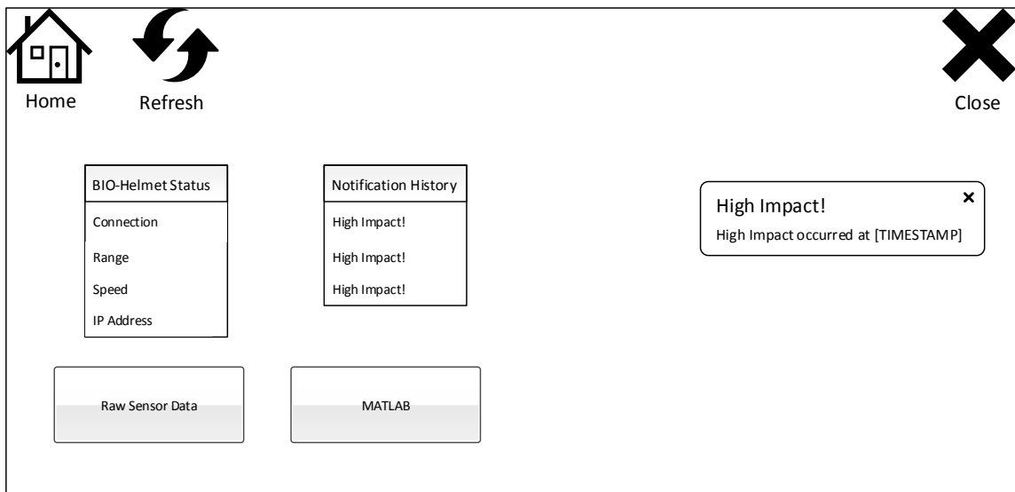
Figure 4-42: Python Graphical User Interface Layout; A figure containing the GUI layout for the main page of the BIO-Helmet graphical user interface
