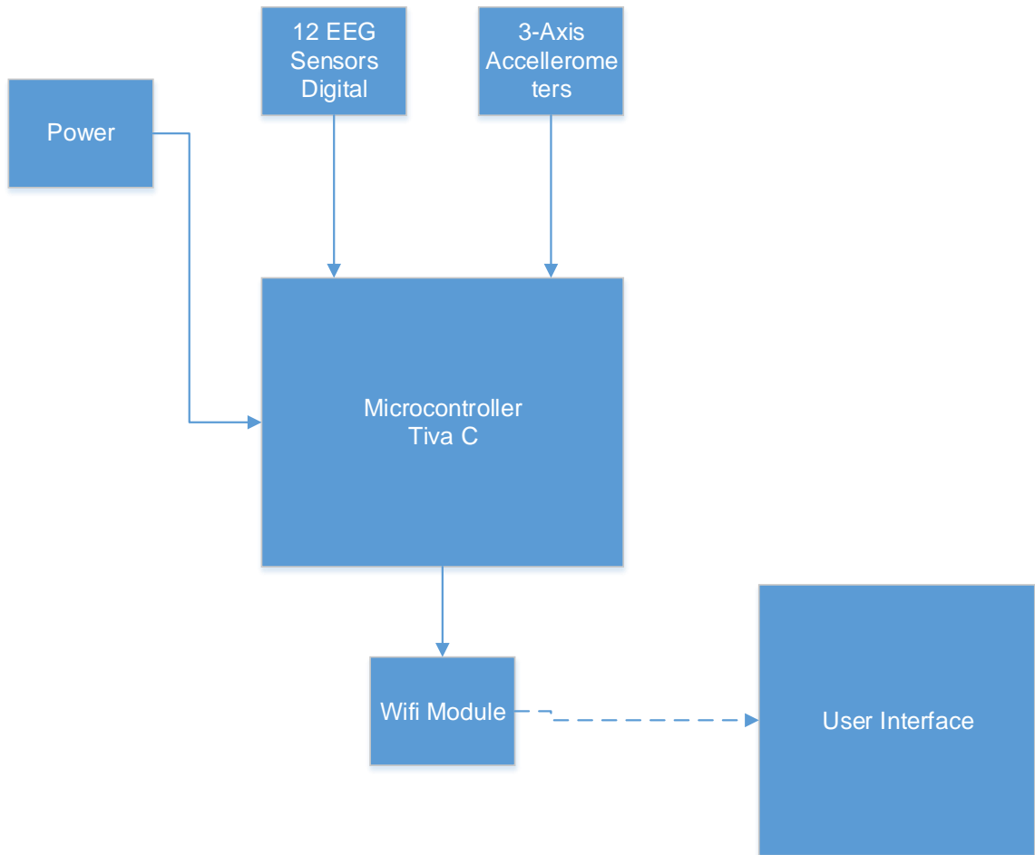
Figure 4-20: Design Layout; The block diagram of the full design layout with all sensors connected
