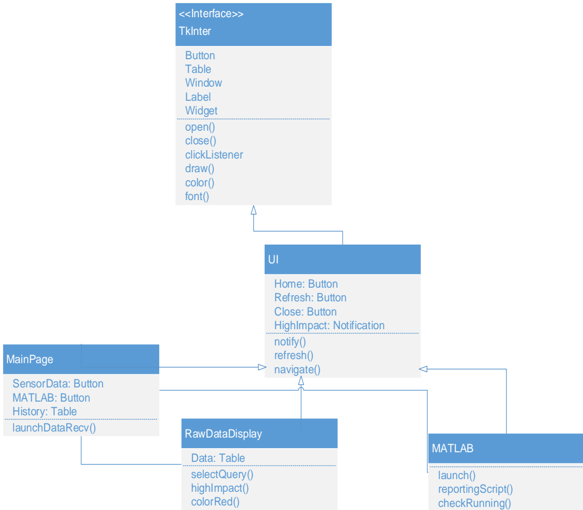
Figure 4-44: Python Graphical Frontend Class Diagram; A UML class diagram representing the implementation of the BIO-Helmet local server GUI
