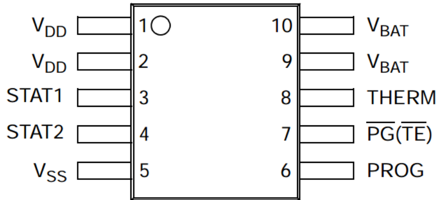
Figure 4-28: MCP73833/4 Pin Layout; A figure demonstrating the pin layout and package description for the MCP73833/4; reprinted with permission from Microchip Technology, Inc.
