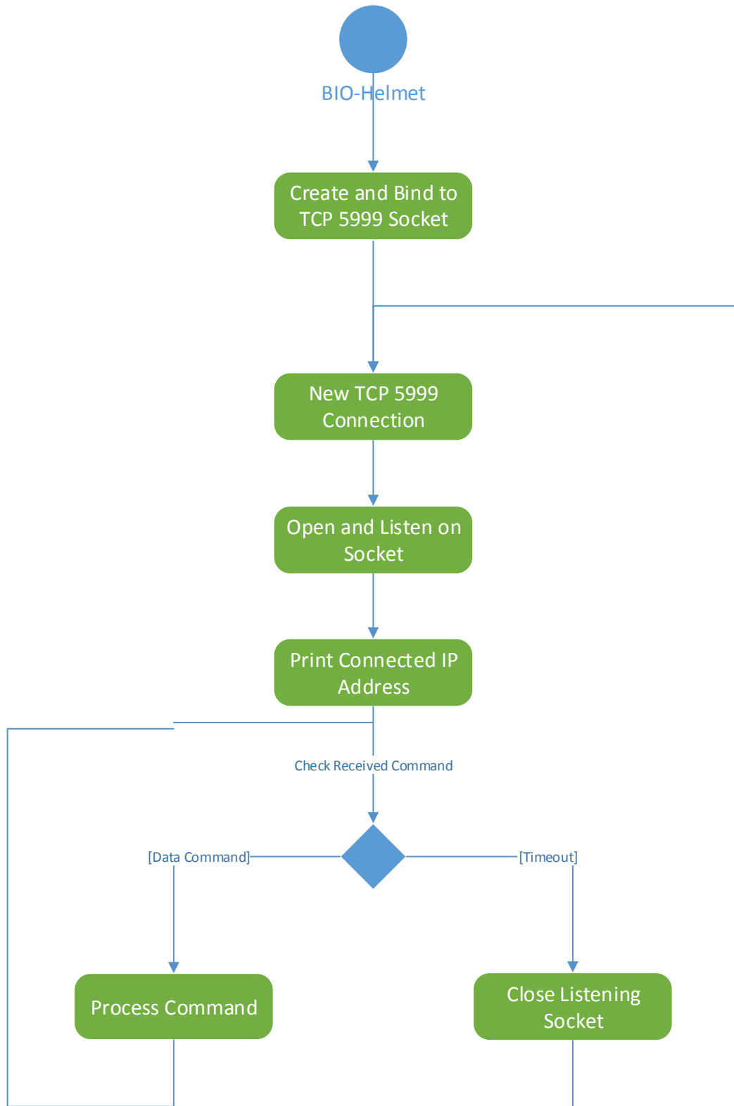
Figure 4-36: Receiving Data Activity Diagram; A UML activity diagram describing the data receiving module of the Python data receiving script
