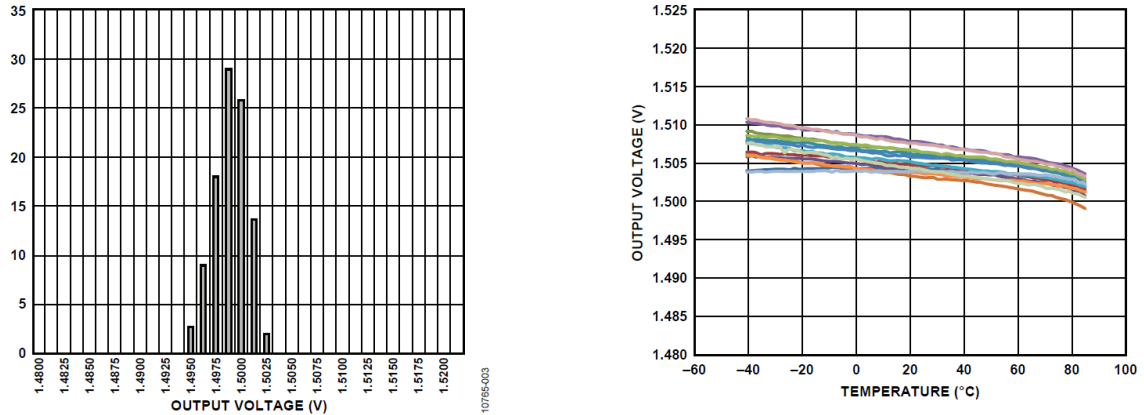
Figure 4-19: ADXL377 Output Inaccuracies; A figure demonstrating the output voltage vs tested population and temperature at 0g and V_s=3V ; reprinted with permission from Analog Devices, Inc.
