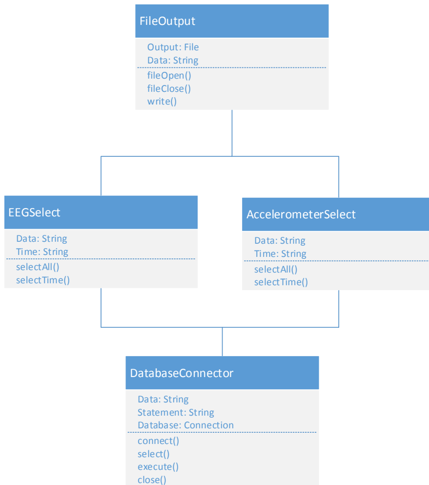
Figure 4-40: Python Data Reporting Script Class Diagram; A figure containing a class diagram for the Python data reporting script
