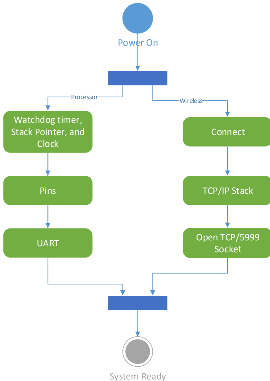
Figure 4-32: BIO-Helmet Initializations; A diagram which describes the order of the initializations when the BIO-Helmet is powered on
