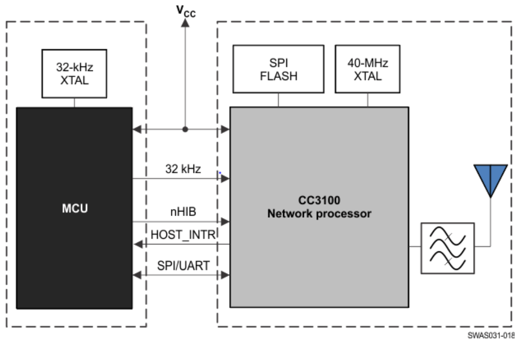
Figure 4-22: CC3100 Modules; A figure describing the major modules present within the CC3100 chip; reprinted with permission from Texas Instruments, Inc.
