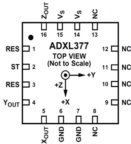
Figure 4-17: ADXL377 Pin Configuration; A figure showing a top down view of the ADXL377 pin configuration; reprinted with permission from Analog Devices, Inc.
