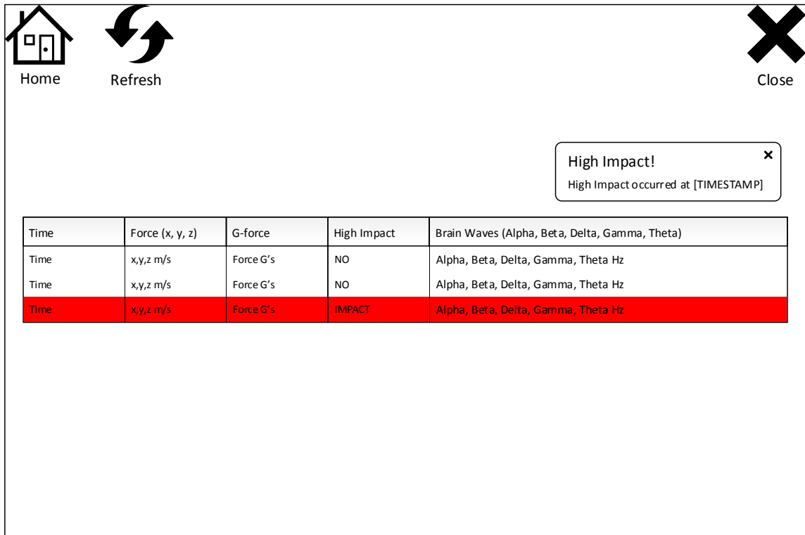
Figure 4-45: Python Graphical User Interface Raw Sensor Data; A figure describing the GUI layout of the raw sensor data display screen of the Python graphical frontend.
