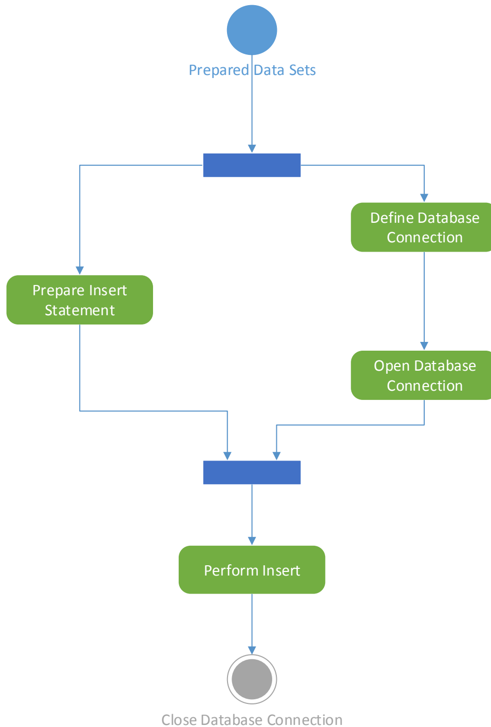
Figure 4-38: SQLite Database Insert Activity Diagram; A UML activity diagram demonstrating the SQLite database insert module of the data receiving Python script
