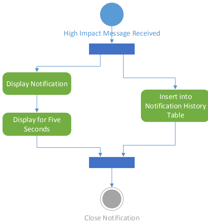
Figure 4-47: High Impact Notification UML; A UML activity diagram describing the high impact notification flow of the Python graphical user frontend
