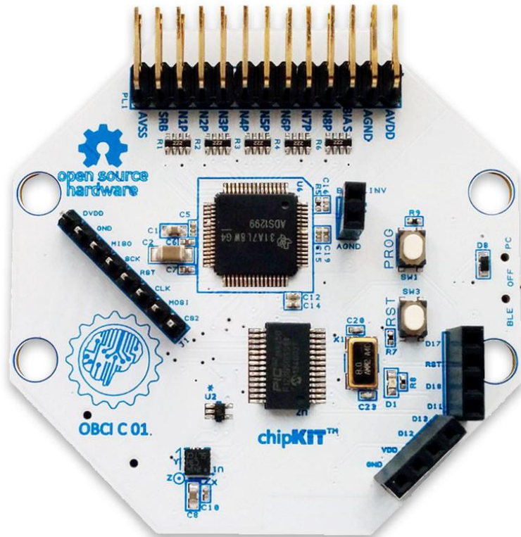
Figure 3-1: OpenBCI Board; An image of the OpenBCI board; reprinted with permission from OpenBCI
