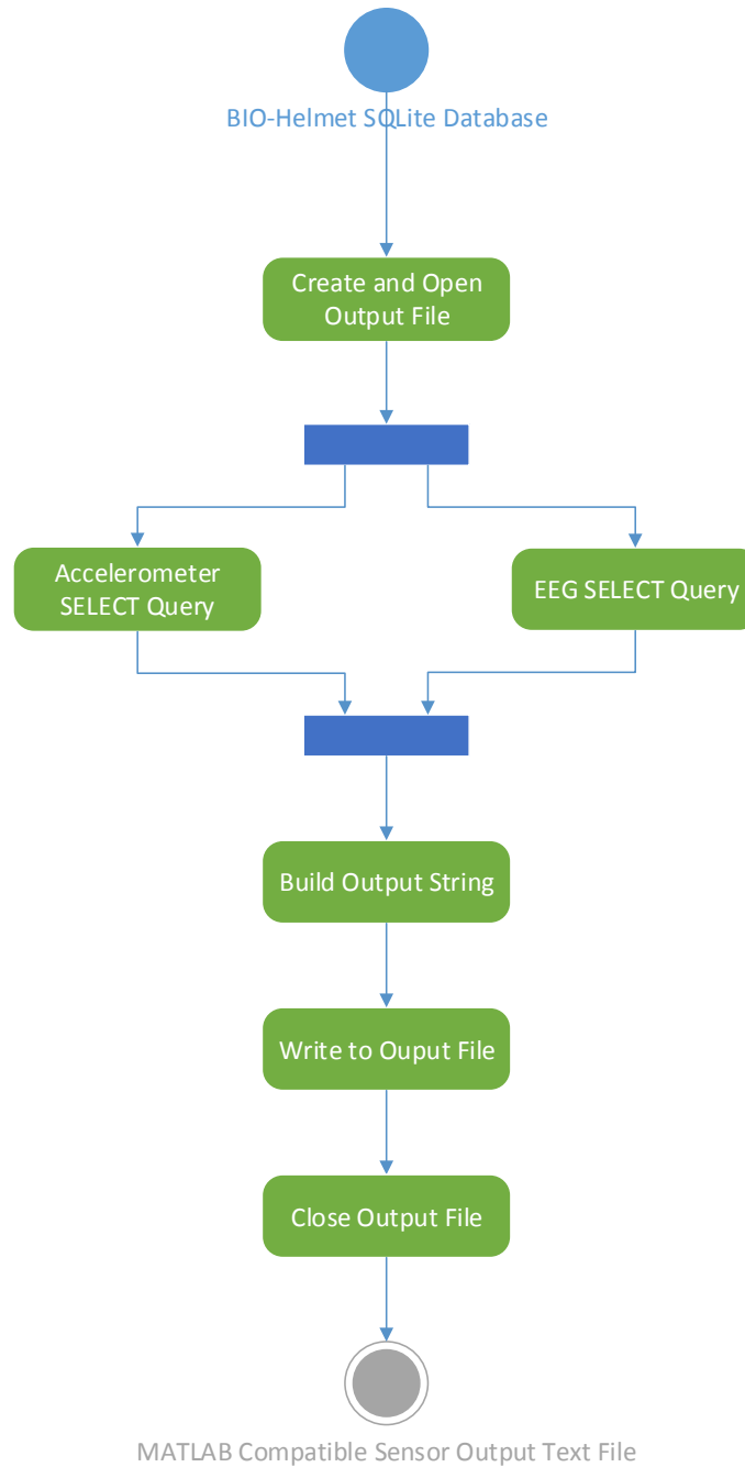
Figure 4-41: Python Data Reporting Script Activity Diagram; A figure containing a UML activity diagram describing the program flow and function
